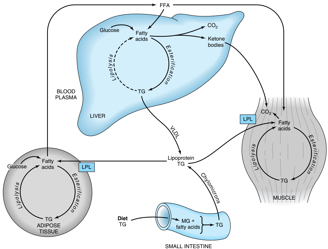
Figure 15–6. Transport and fate of major lipid substrates and metabolites. (FFA, free fatty acids; LPL, lipoprotein lipase; MG, monoacylglycerol; TG, triacylglycerol; VLDL, very low density lipoprotein.)
