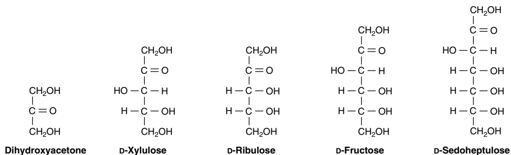
Figure 13-7. Examples of ketoses of physiological significance.
