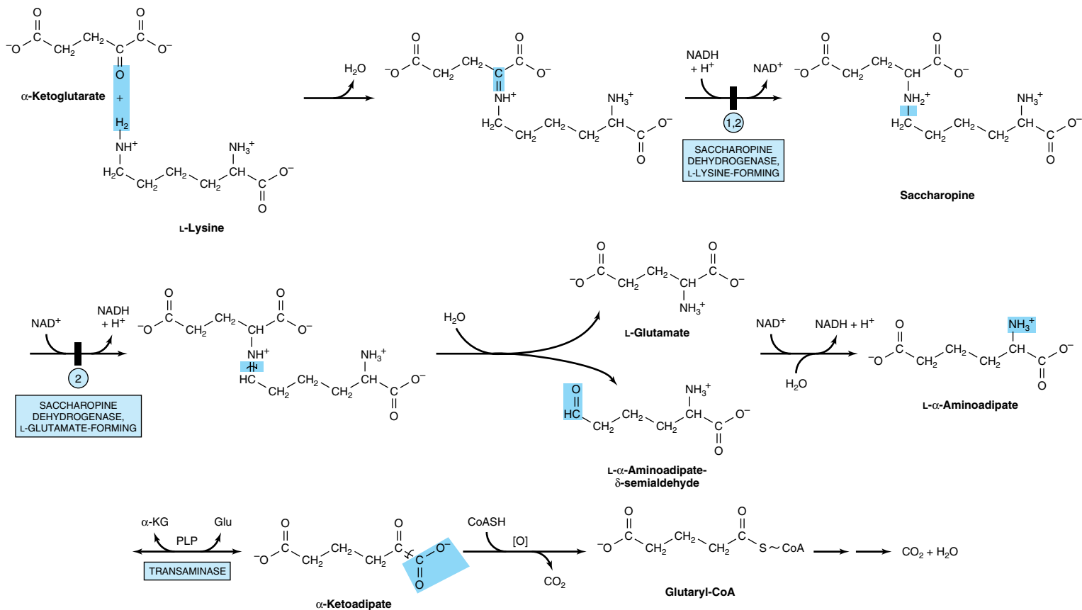
Figure 30–14. Catabolism of L-lysine. (α-KG, α-ketoglutarate; Glu, glutamate; PLP, pyridoxal phosphate.) Circled numerals indicate the probable sites of the metabolic defects in ① periodic hyperlysinemia with associated hyperammonemia; and ② persistent hyperlysinemia without associated hyperammonemia.
