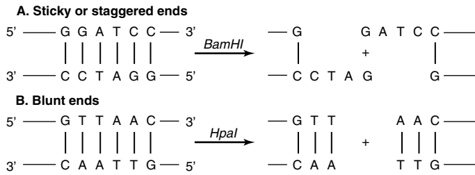
Figure 40–2. Results of restriction endonuclease digestion. Digestion with a restriction endonuclease can result in the formation of DNA fragments with sticky, or cohesive, ends (A) or blunt ends (B). This is an important consideration in devising cloning strategies.
