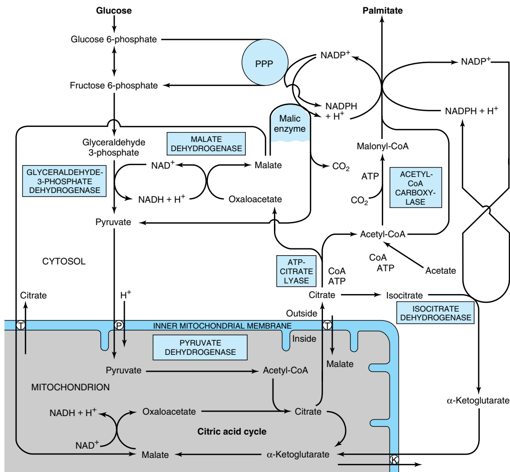
Figure 21–4. The provision of acetyl-CoA and NADPH for lipogenesis. (PPP, pentose phosphate pathway; T, tricarboxylate transporter; K, \alpha -ketoglutarate transporter; P, pyruvate transporter.)
